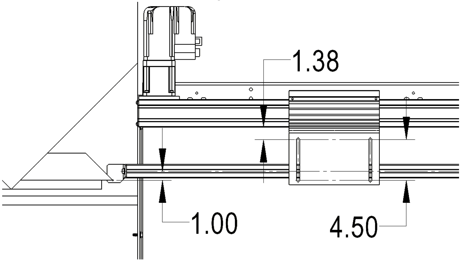
TOP VIEW
